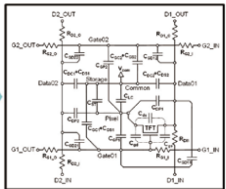
Equivalent Circuit
