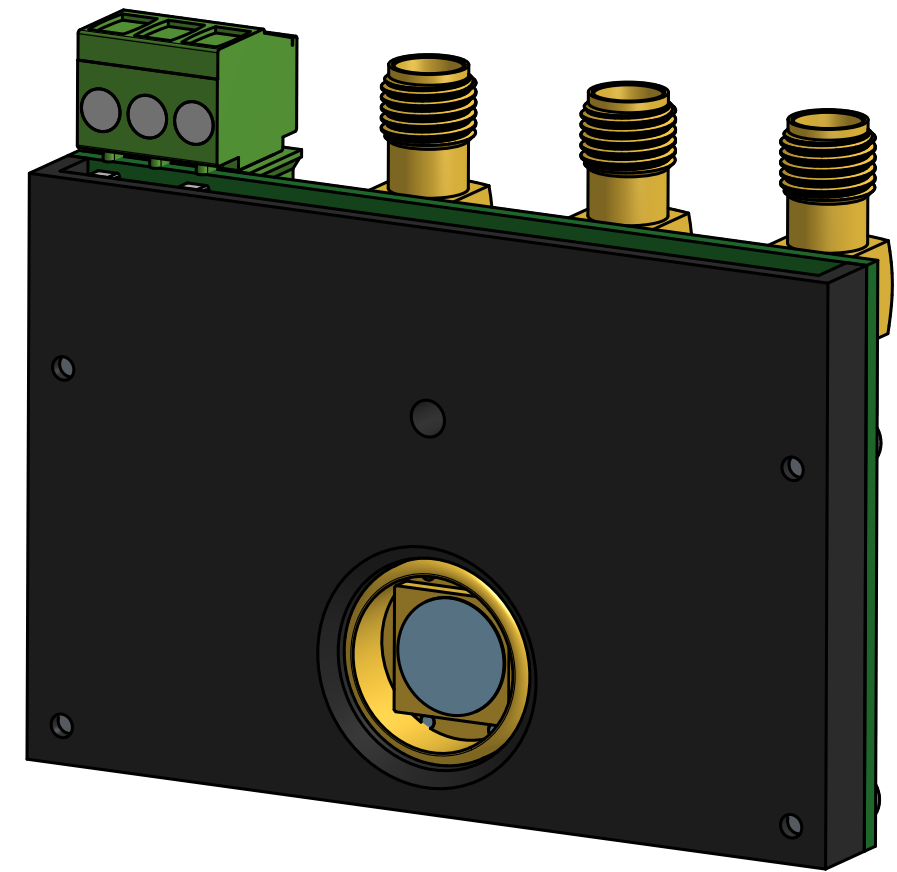
PHOTODIODE DETAIL
