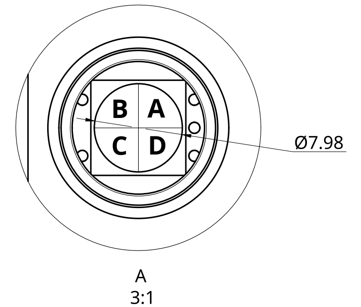
PHOTODIODE DETAIL
