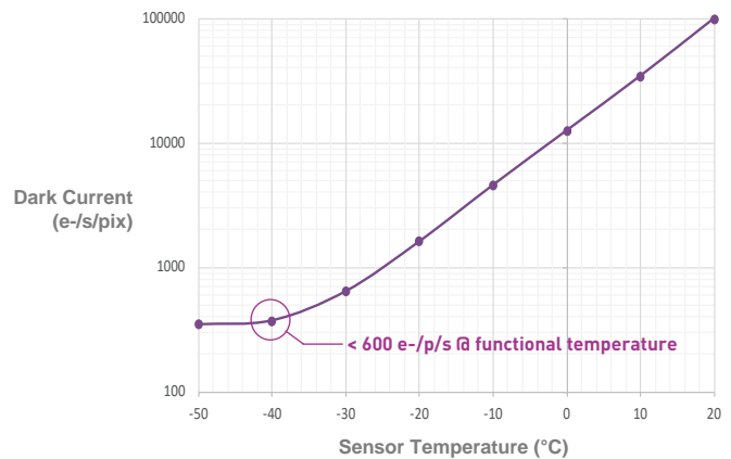
DARK VS SENSOR TEMPERATURE
