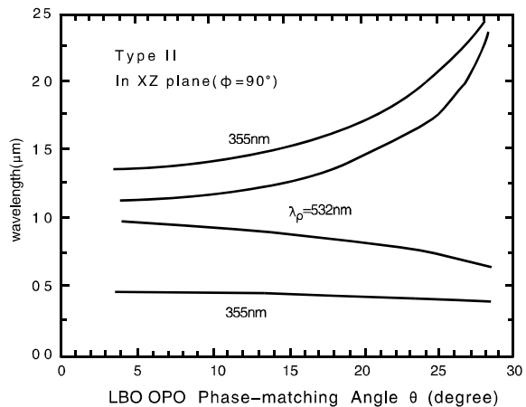
Figure 5. Type II OPO tuning curves of LBO
