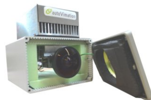
The mount guarantees excellent thermal connection
