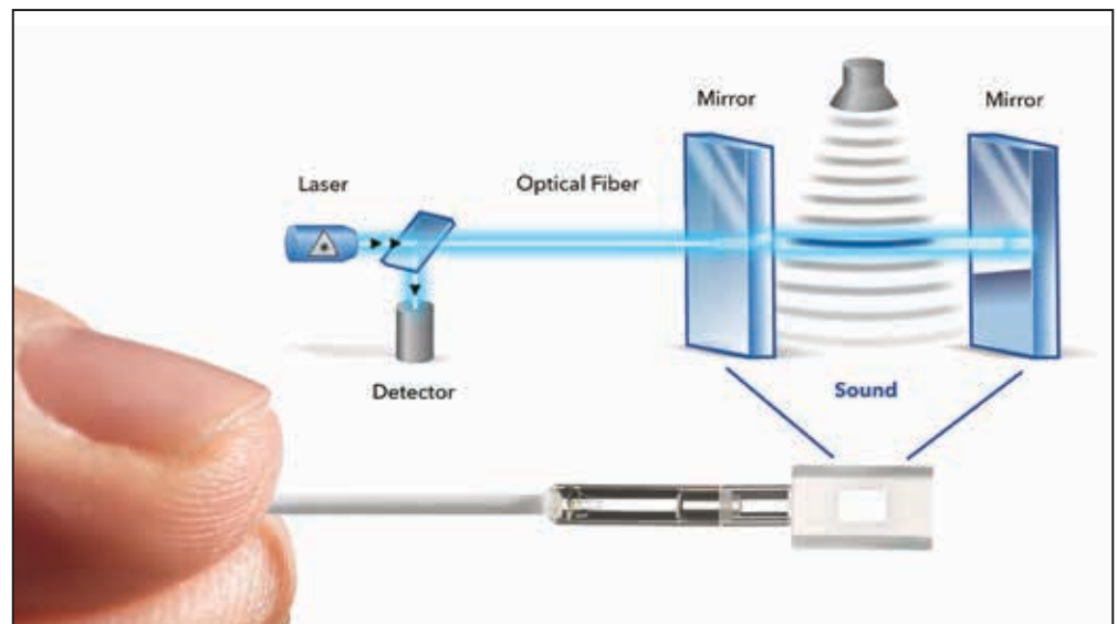
Figure 1 Sensing principle of the optical microphone.
