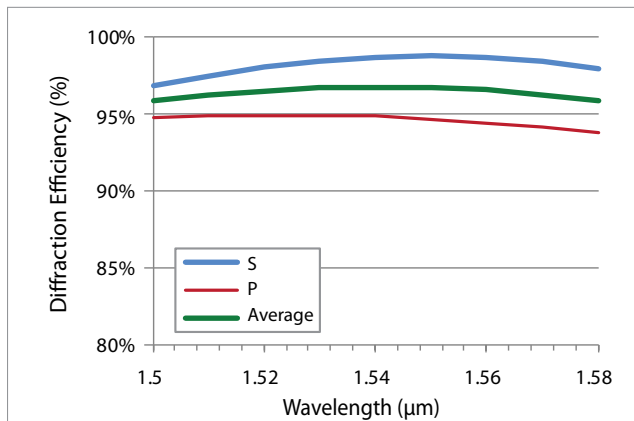
Typical absolute diffraction efficiency at AOI 50.6° *
