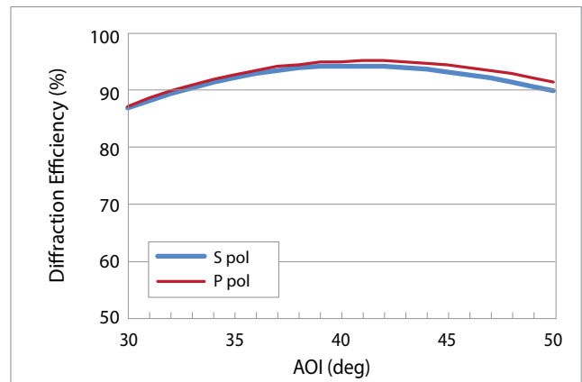
Diffraction efficiency at 875 nm as a function of AOI *
