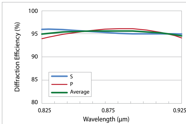
Typical absolute diffraction efficiency at AOI 41.1° *
