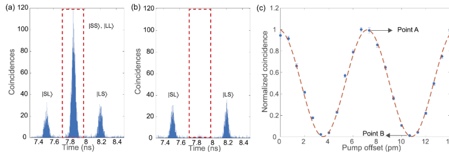
Figure 3: (From R. Dalidet et al. [2]) Interference measurements of the generated photon pairs, demonstrating energy-time entanglement. Shown are coincidence histograms for (a) constructive interference, with a pump offset of 7.35 pm, and (b) destructive interference with a pump offset of 10.65 pm, as well as (c) the interference fringes as a function of pump offset.
