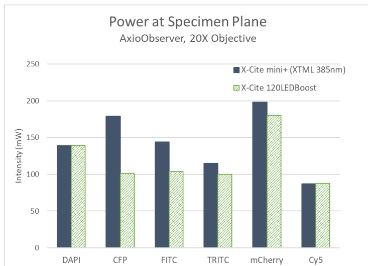
Figure 2: Power comparison at specimen plane using standard filter cubes. X-Cite mini+ matches or exceeds performance of X-Cite 120LEDBoost in all areas of the spectrum.
