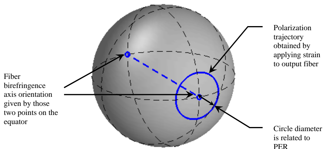
Figure 1: Illustration of the PER measurement method with the polarization analyzer on the Poincaré sphere. The input polarization state into the component is aligned with the PM fiber axis and has a high PER (~30dB). By varying the strain on the output fiber of a component (by applying heat), the polarization state goes through all possible phase differences between the two orthogonal proper polarizations of the system. This draws the blue circle on the Poincaré sphere. The diameter of the circle yields the PER with respect to the fiber axis. The two points linked with a dashed line, one of which is in the center of the polarization trajectory, represent the orientation of the two proper axes of the fiber.
