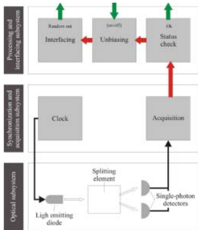
Figure 2: Block diagram of the Quantis random number generator.
