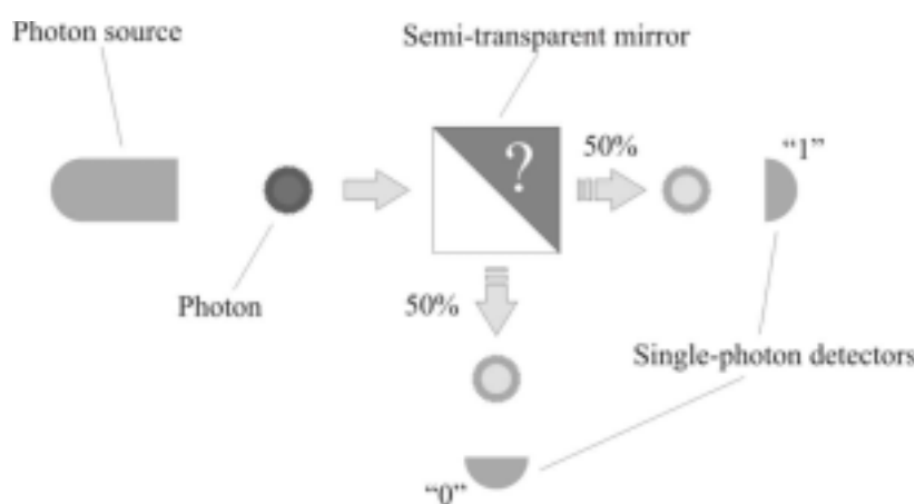
Figure 1: Optical system used to generate random numbers.
