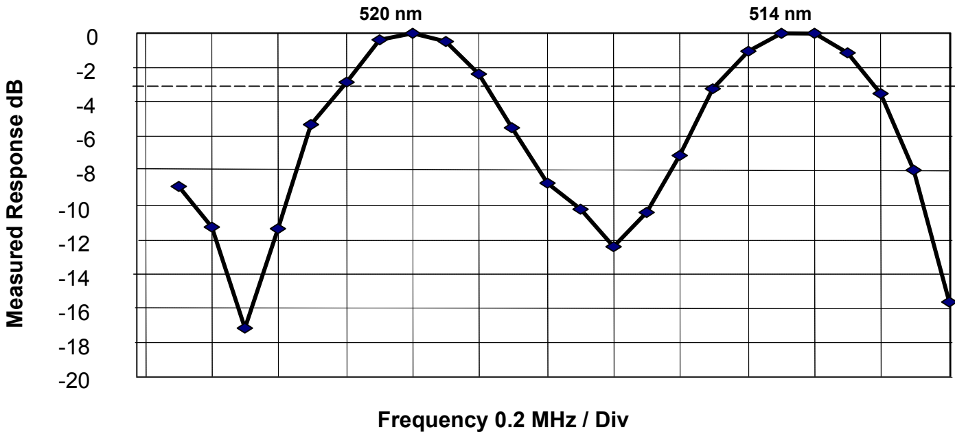
Figure 6 48058 Frequency Response
