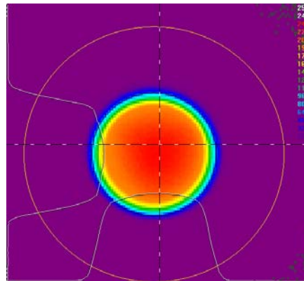
2mm x 63 mm rod, 0.6% doped Nd:YAG
